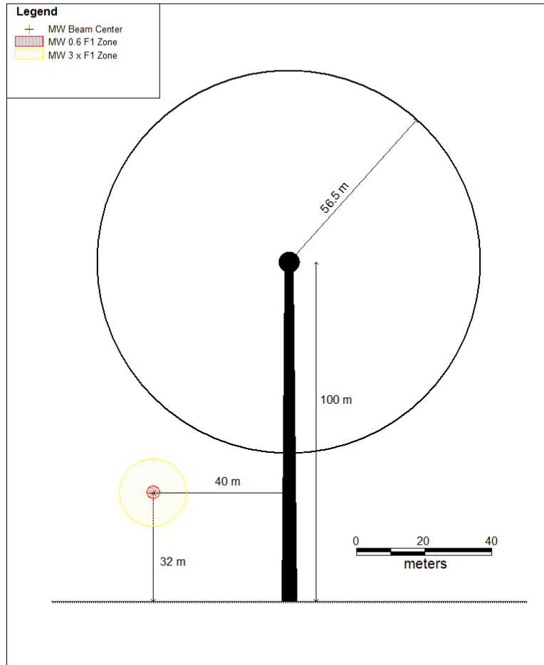
Figure 1: T-4 wind turbine vs microwave link consultation zone
