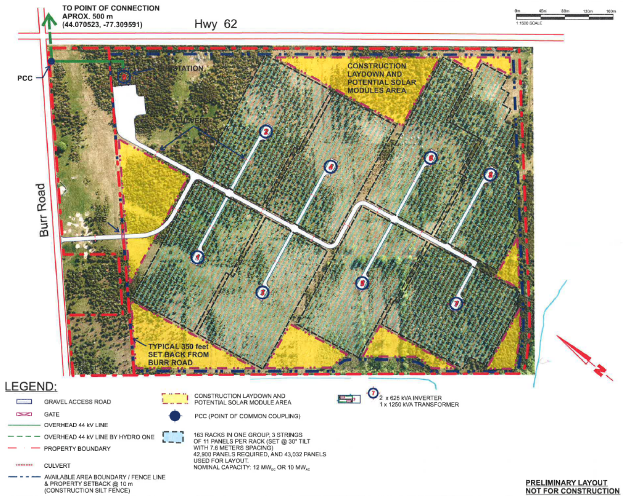
Figure 1: Site Layout
